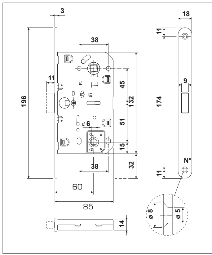
Product Dimensions
