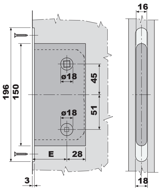
Drilling Diagram
